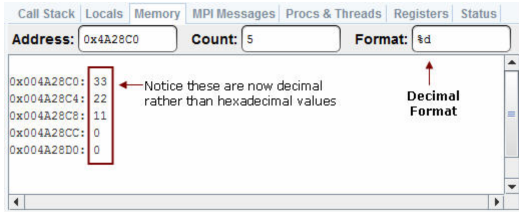
Figure 17 Memory Tab in Decimal Format
