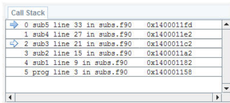
Figure 14 Call Stack Outside Current Frame
