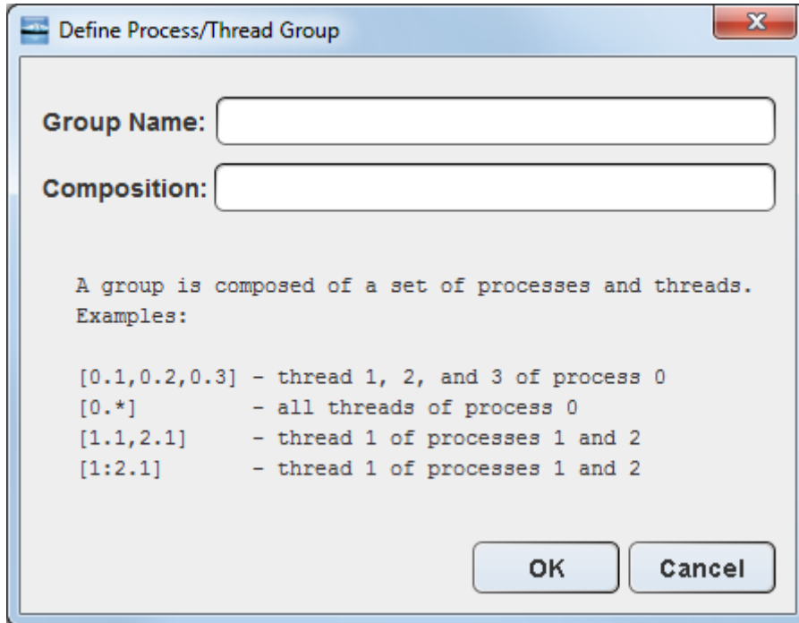
Figure 23 Process/Thread Group Dialog Box
