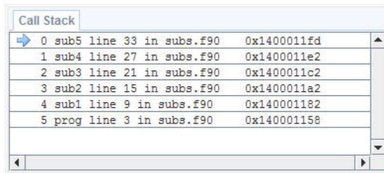
Figure 13 Call Stack Tab
