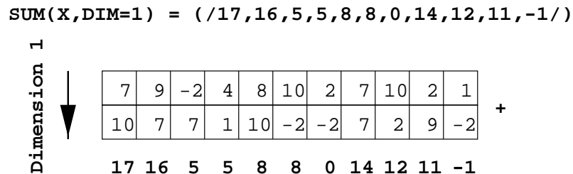
Figure 19: Summing along Dimension 1 of a 2D Array
